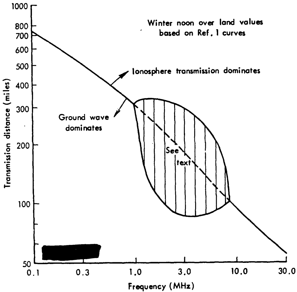
Fig. 5-1 Comparative ground wave and ionospheric transmission
